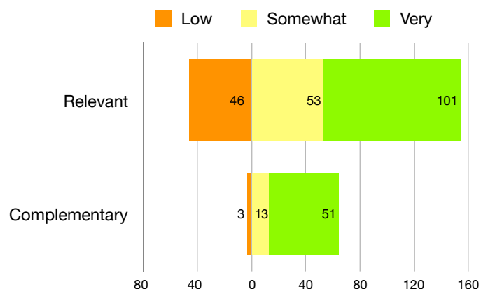
Fig. 12. RQ 4 : Relevance of Stack Overflow discussions to video fragments, and complementariness to videos.
