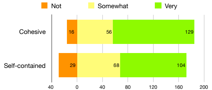
Fig. 11. RQ 3 : Distribution of cohesiveness and self-containment.
